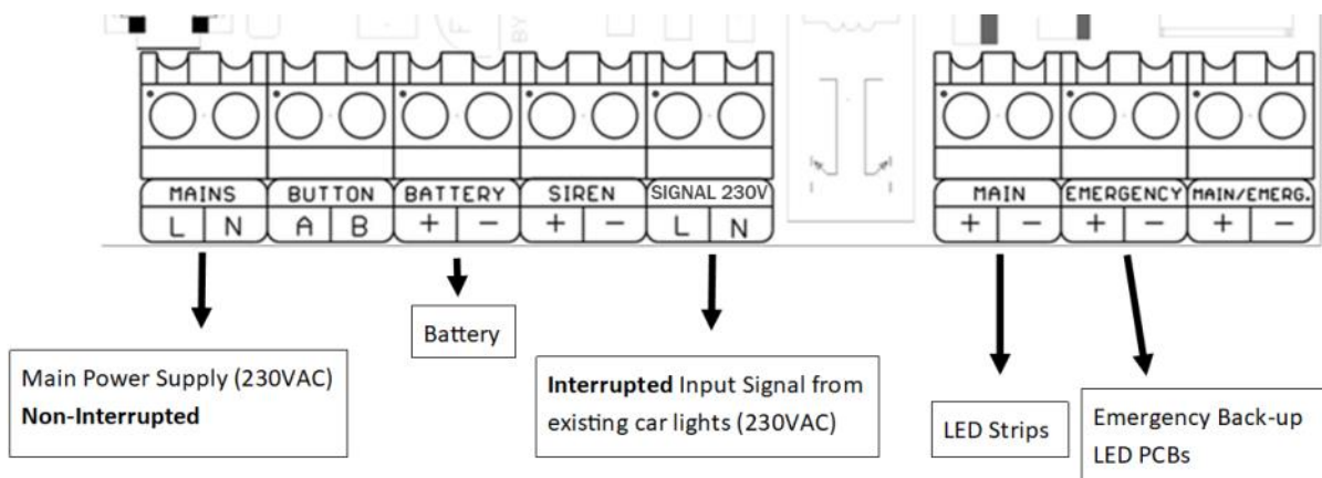
Figure 1. FRWD0805 typical connection diagram.
